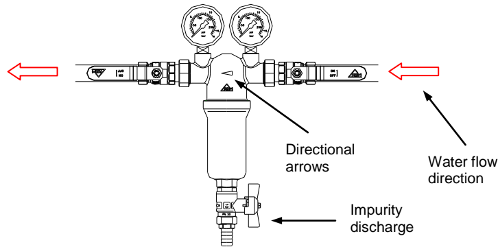
Assembly diagram of the self-cleaning filter inside a hydraulic circuit
