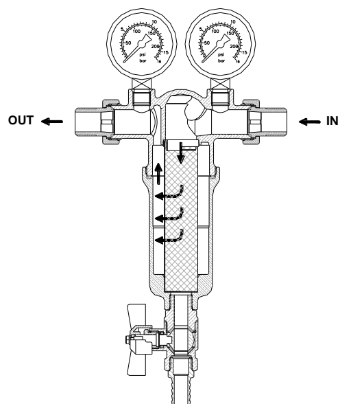
Diagram of water passing through the filter
