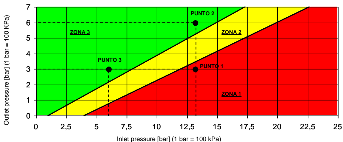
CAVITATION DIAGRAM *
